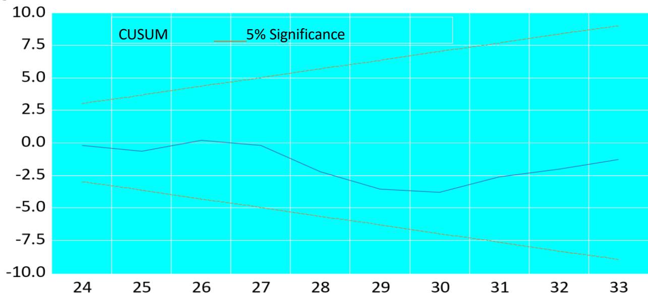
Figure 1: CUSUM Test Results
